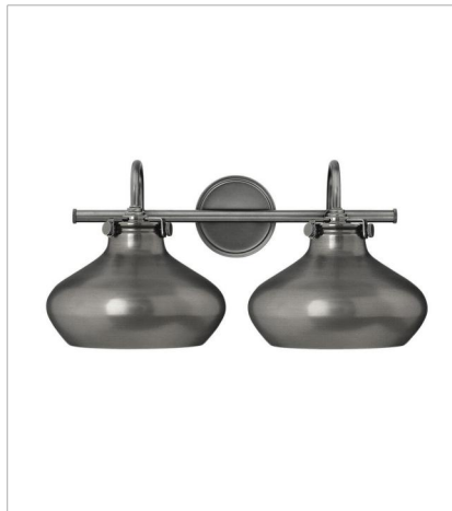
50028AN METAL SHADE TWO LIGHT VANITY 21" W, 10.5" H Socketed
